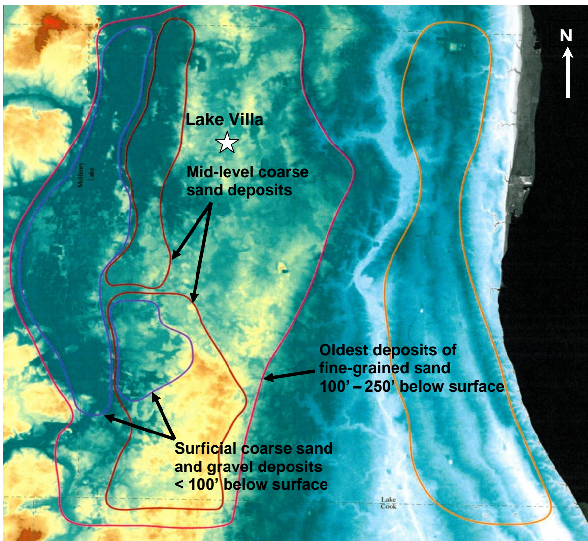
FIGURE 3 Shallow Subsurface Geology of Lake County
